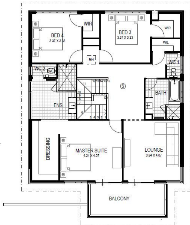
UPPER FLOOR PLAN SCALE 1:100
