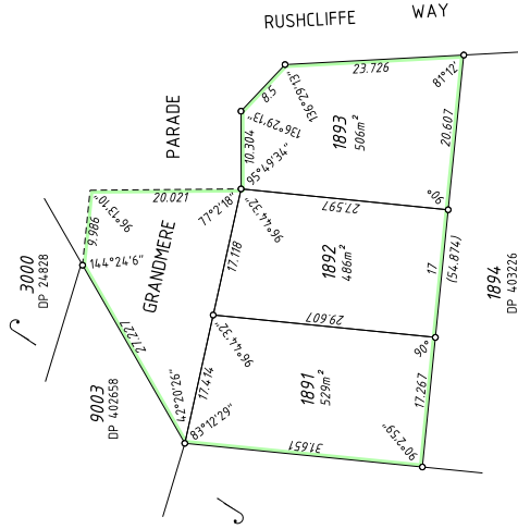
ENLARGEMENT AT 'A' NOT TO SCALE
