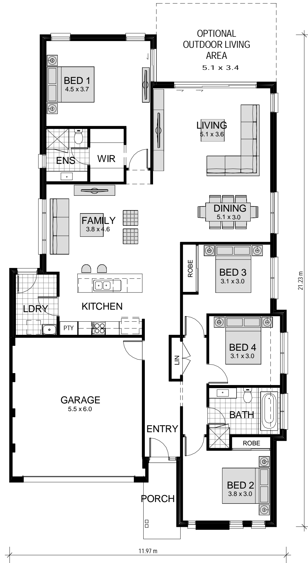
GROUND FLOOR
