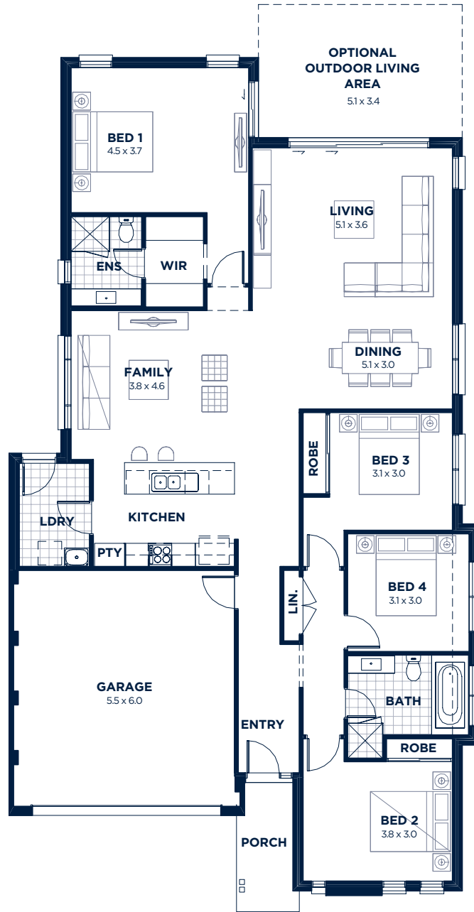
FLOOR PLAN
