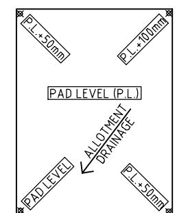
TYPICAL ALLOTMENT GRADING DETAIL
