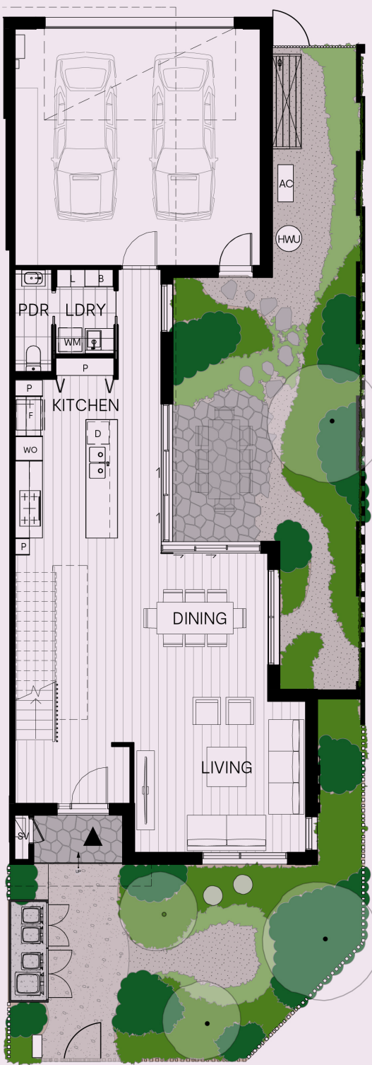
Ground floor
