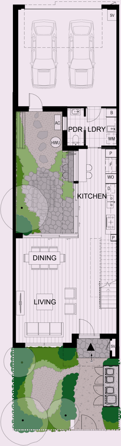
Ground floor
