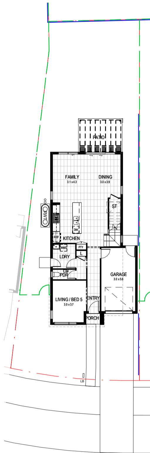
SPINNAKER DRIVE GROUND FLOOR PLAN
